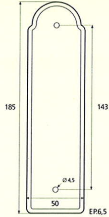
demi plaque Louis XVI
