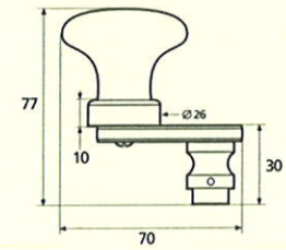
manivelle bordelaise tradition
