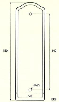
demi plaque bois
